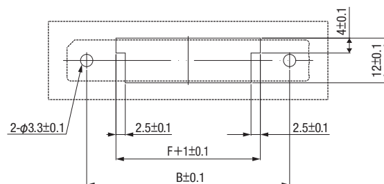
▶ Panel layout (Component side view)
