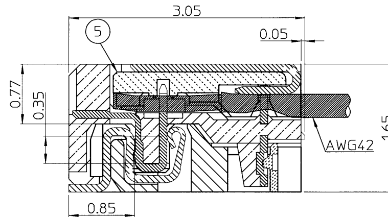
X-X' mated cross section(20:1) USLS00-30-X/USLS20-30
